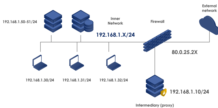
Figure 4. Network diagram
